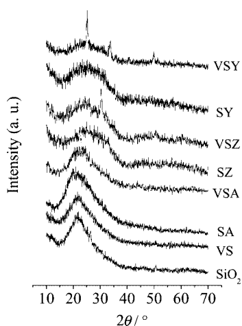
Figure 1. Powder X-ray diffraction patterns of SiO 2 , modified silica samples and vanadia impregnated samples.
