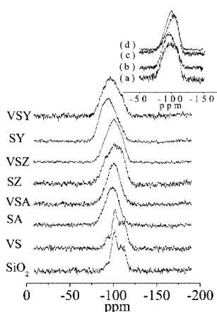
Figure 3. ^1H \rightarrow ^{29}Si CP MAS NMR spectra of SiO_2 , modified silica samples and vanadia impregnated samples. Inset shows the ^{29}Si single pulse and CP MAS NMR spectra, respectively, for VSX (a and b) and VSZ (c and d).
