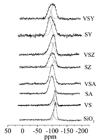
Figure 2. Deconvoluted 29 Si MAS NMR spectra of SiO 2 , modified silica samples and vanadia impregnated samples.
