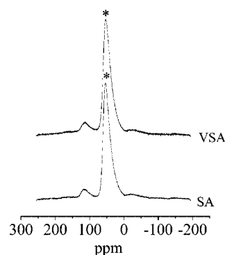
Figure 4. ^{27}Al MAS NMR spectra of SA and VSA samples (the peak marked with an asterisk is the isotropic peak).
