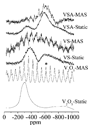
Figure 6. ^{51}\text{V} static and MAS NMR spectra of \text{V}_2\text{O}_5 , VS and VSA (the peak marked with an asterisk is the isotropic peak).
