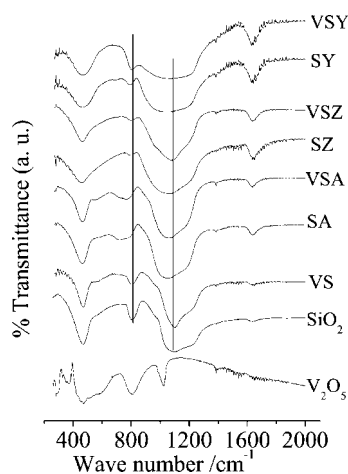
Figure 5. IR spectra of \text{V}_2\text{O}_5 , \text{SiO}_2 , modified silica samples and vanadia impregnated samples.
