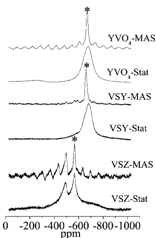
Figure 7. ^{51}\text{V} static and MAS NMR spectra of VSZ, VSY and \text{YVO}_4 samples (the peak marked with an asterisk is the isotropic peak).
